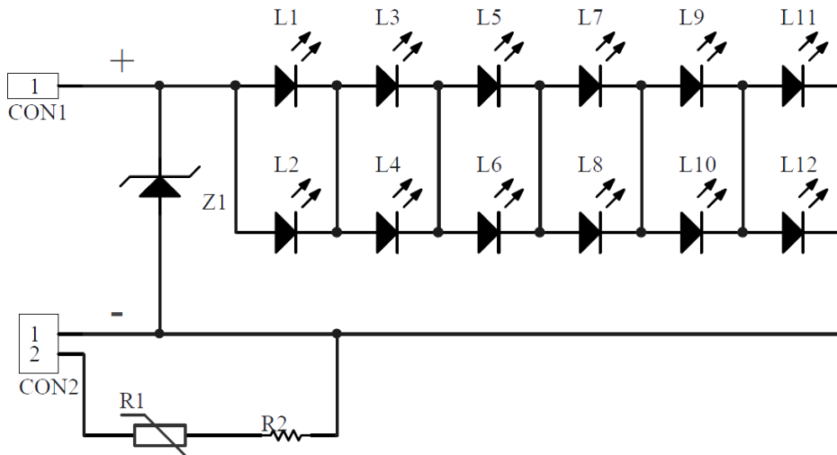
Fig 10. circuit drawing
